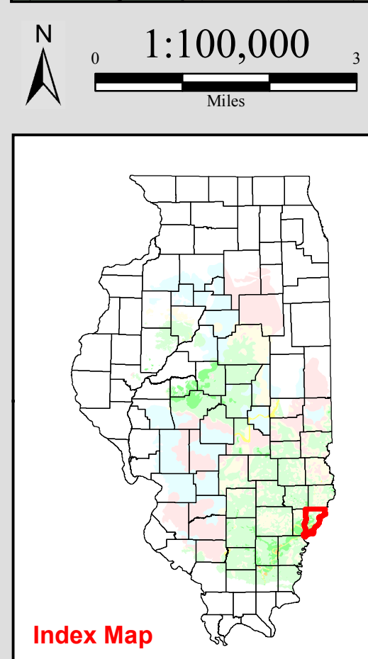
Fig. 1 The Springfield Coal underlies about two thirds of Illinois as well as portions of western Indiana and western Kentucky. The coal crops out along the margins of the Illinois Basin and reaches a maximum depth in Illinois of about 1,300 feet. (See Fig. 1, and Fig. 2.) The Springfield Coal is in the Carboniferous formation which is part of the Desmoinesian Series. (See Fig. 4) The Springfield Coal is normally overlain by a black fissile shale called the Turner Mine shale, but in southeastern Illinois, in a belt several miles wide that trends southwestward, the coal is thick and is overlain by the gray silty Dykersburg Shale. In that belt the coal is commonly split by shale partings, and contains less pyrite than where it is overlain by the black fissile shale (Hopkins, 1968 - 1993). (See Fig. 4.)
