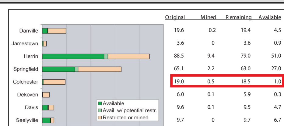
Fig. 3 The Colchester Coal underlies much of Illinois as well as portions of western Indiana and western Kentucky. The coal crops out along the margins of the Illinois Basin and reaches a maximum depth in Illinois of about 1,500 feet. (See Fig. 1 and Fig. 2) The Colchester Coal and its overlying black shale, the Mecca Quarry Shale, are part of the Carboniferous formation of the Desmoinesian Series (See Fig. 4) and are key marker beds that have been traced throughout the basin. In southern, central, and eastern Illinois, the Colchester is generally thin, ranging from less than one inch to 18 inches thick. Throughout most of its northern and western extent, the Colchester is 2 to 3.5 feet thick (locally 4 feet) where it has been mined. The Colchester Coal is perhaps the most widespread minable seam in North America and is correlated with the Crowburg Coal of Missouri and Kansas, the Schultzown Coal Member (Ill.) of Indiana, the Lower Kittanning Coal of Ohio, the Princess No. 6 of eastern Kentucky, and the No. 6 Block of West Virginia.
