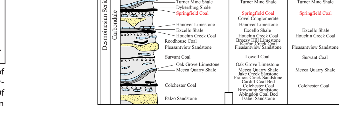
Fig. 4 Pennsylvanian Stratigraphic Column
