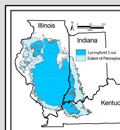
Fig. 1 The Springfield Coal underlies about two thirds of Illinois as well as portions of western Indiana and western Kentucky. The coal crops out along the margins of the Illinois Basin and reaches a maximum depth in Illinois of about 1,300 feet. (See Fig. 1 and Fig. 2) The Springfield Coal is in the Carboniferous formation which is part of the Desmonian Series. (See Fig. 4) The Springfield Coal is normally overlain by a black fissile shale called the Turner Mine shale, but in southeastern Illinois, in a belt several miles wide that trends southwestward, the coal is thick and is overlain by the gray silty Dykersburg Shale. In that belt the coal is commonly split by shale partings, and contains less pyrite than where it is overlain by the black fissile shale (Hopkins, 1968-1995). (See Fig. 4.)
