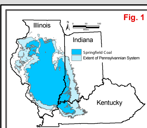
by the gray silty Dykersburg Shale. In that belt the coal is commonly split by shale partings, and contains less pyrite than where it is overlain by the black fissile shale (Hopkins, 1968 - B95). (See Fig 4.)
