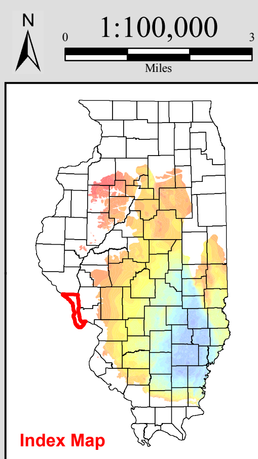
by the gray silty Dykersburg Shale. In that belt the coal is commonly split by shale partings, and contains less pyrite than where it is overlain by the black fissile shale (Hopkins, 1968 - B95). (See Fig 4.)
