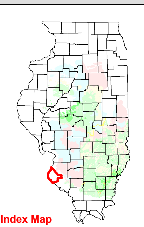
Fig. 1 The Springfield Coal underlies about two-thirds of Illinois as well as portions of western Indiana and western Kentucky. The coal crops out along the margins of the Illinois Basin and reaches a maximum depth in Illinois of about 1,300 feet. (See Fig. 1, and Fig. 2.) The Springfield Coal is in the Carbonate formation which is part of the Des Moines Series. (See Fig. 4) The Springfield Coal is normally overlain by a black fissile shale called the Turner Mine shale, but in southeastern Illinois, in a belt several miles wide that trends southwestward, the coal is thick and is overlain by the gray silty Dykersburg Shale. In that belt the coal is commonly split by shale partings, and contains less pyrite than where it is overlain by the black fissile shale (Hopkins, 1968-1955). (See Fig. 4.)
