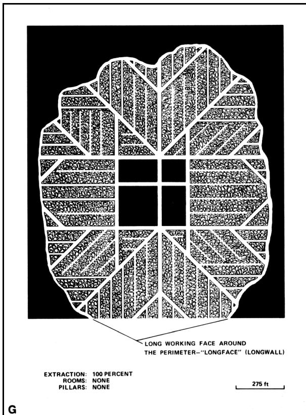
Figure 1 (cont'd) Mining methods: (E) checkerboard room and pillar (CRP), (F) high extraction retreat (HER), (G) early (pre-1960) longwall, (H) post-1959 longwall.
