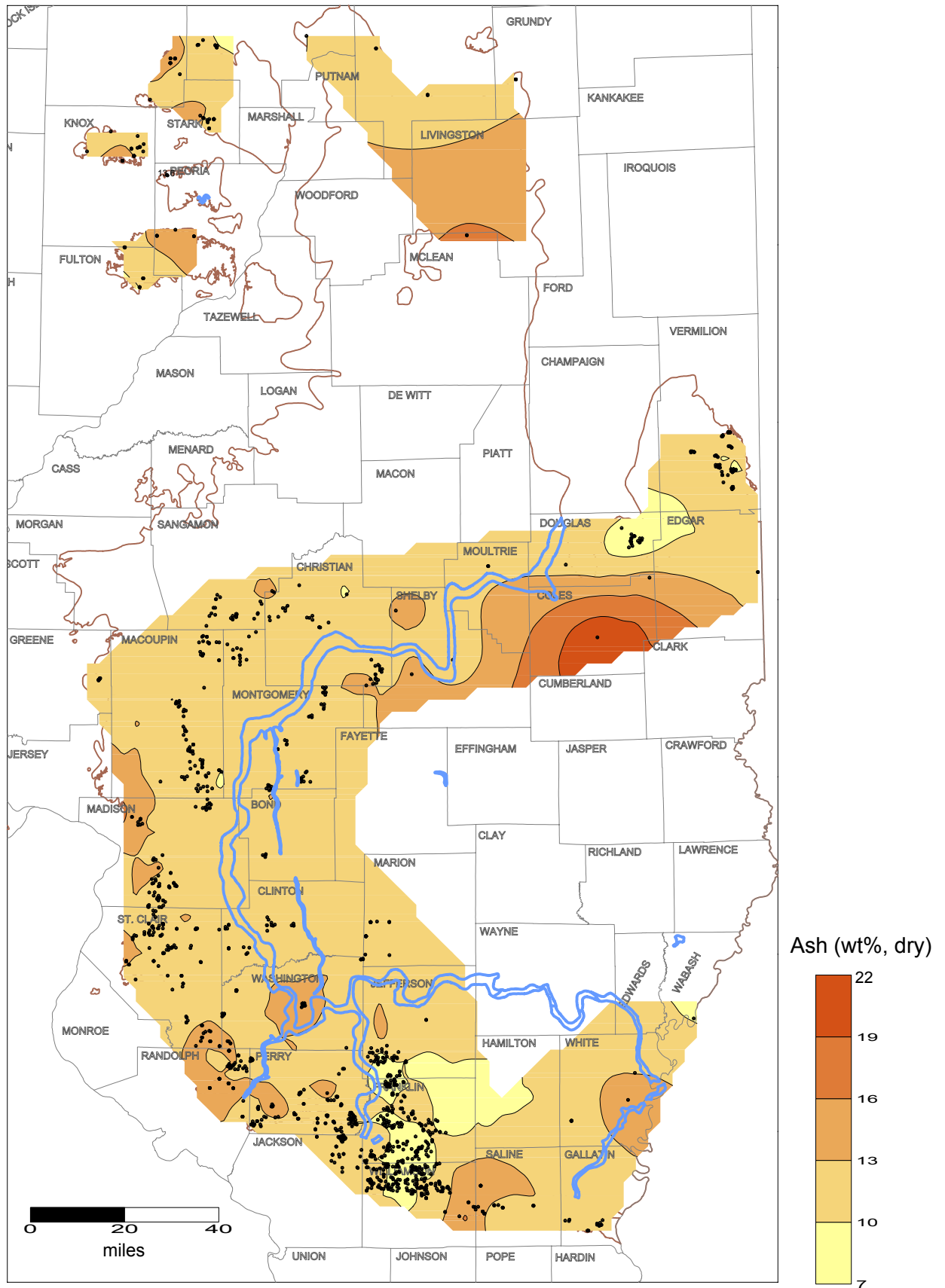
Ash yield of Herrin Coal seam in Illinois. Black solid circles indicate sample locations. Brown and blue lines indicate the limit of the Herrin seam and Walshville channel, respectively.
