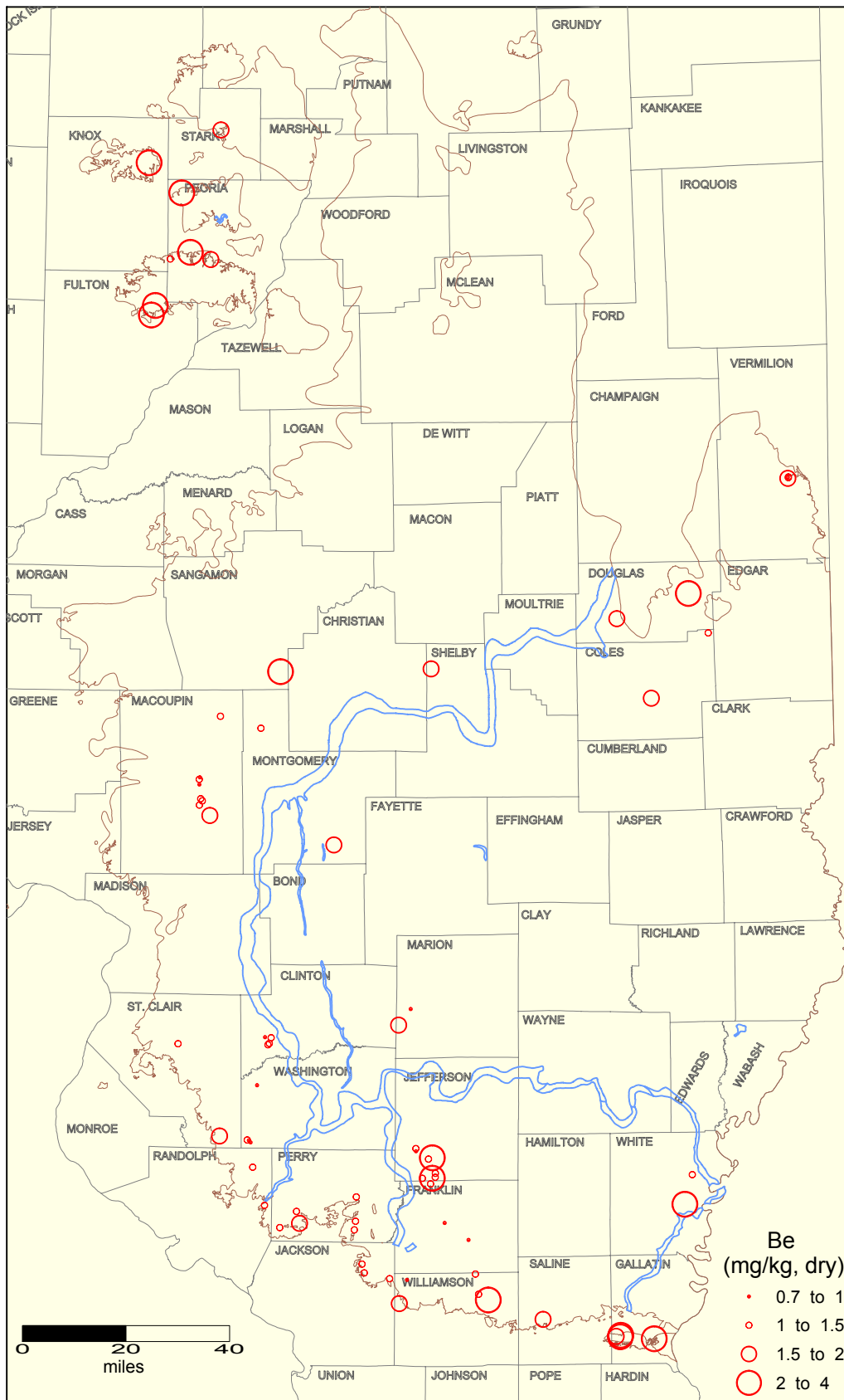
Beryllium concentration in Herrin Coal seam in Illinois. Brown and blue lines indicate the limit of the Herrin seam and Walshville channel, respectively.
