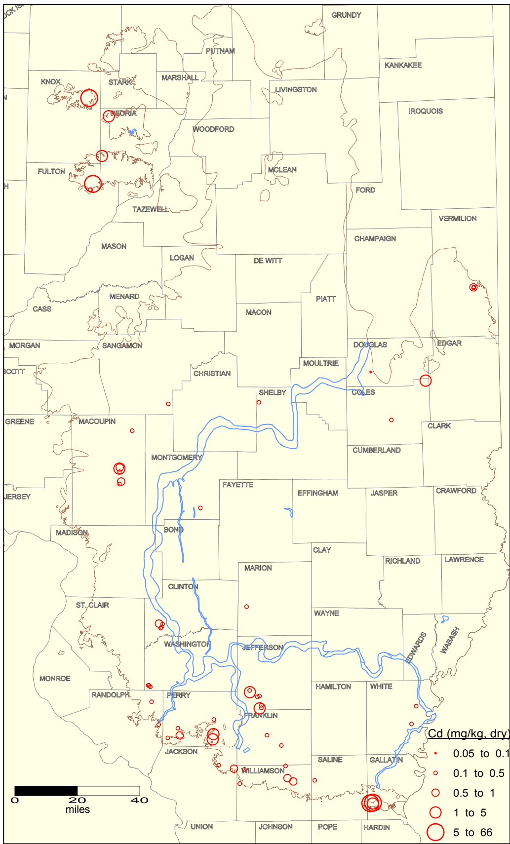
Cadmium concentration in Herrin Coal seam in Illinois. Brown and blue lines indicate the limit of the Herrin seam and Walshville channel, respectively.
