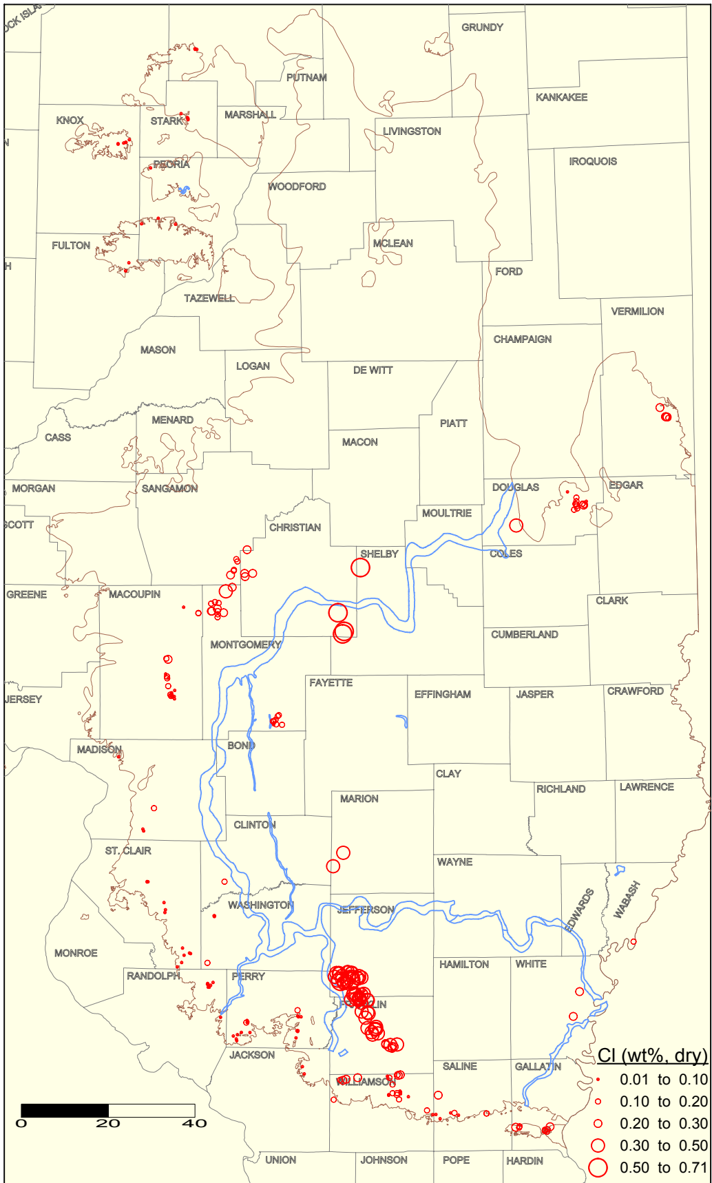
Chlorine content of Herrin Coal seam in Illinois. Brown and blue lines indicate the limit of the Herrin seam and Walshville channel, respectively.
