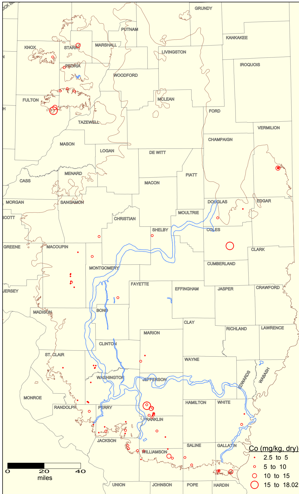
Cobalt concentration in Herrin Coal seam in Illinois. Brown and blue lines indicate the limit of the Herrin seam and Walshville channel, respectively.
