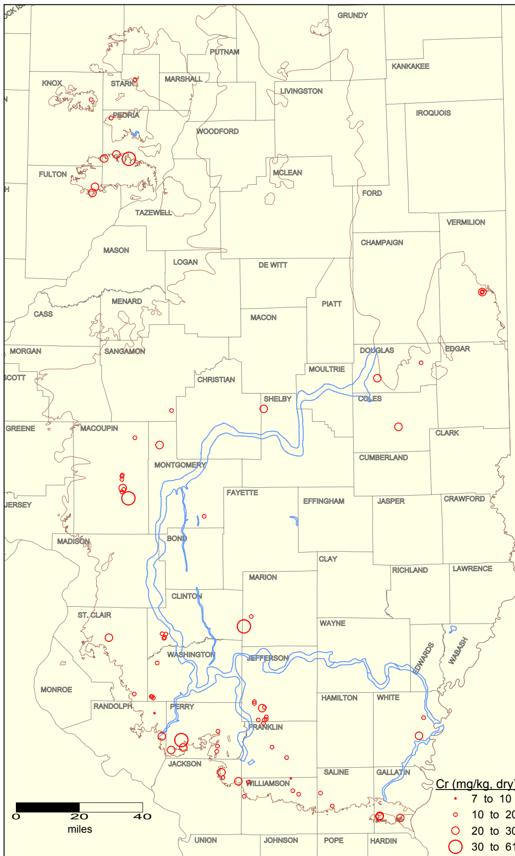
Chromium concentration in Herrin Coal seam in Illinois. Brown and blue lines indicate the limit of the Herrin seam and Walshville channel, respectively.
