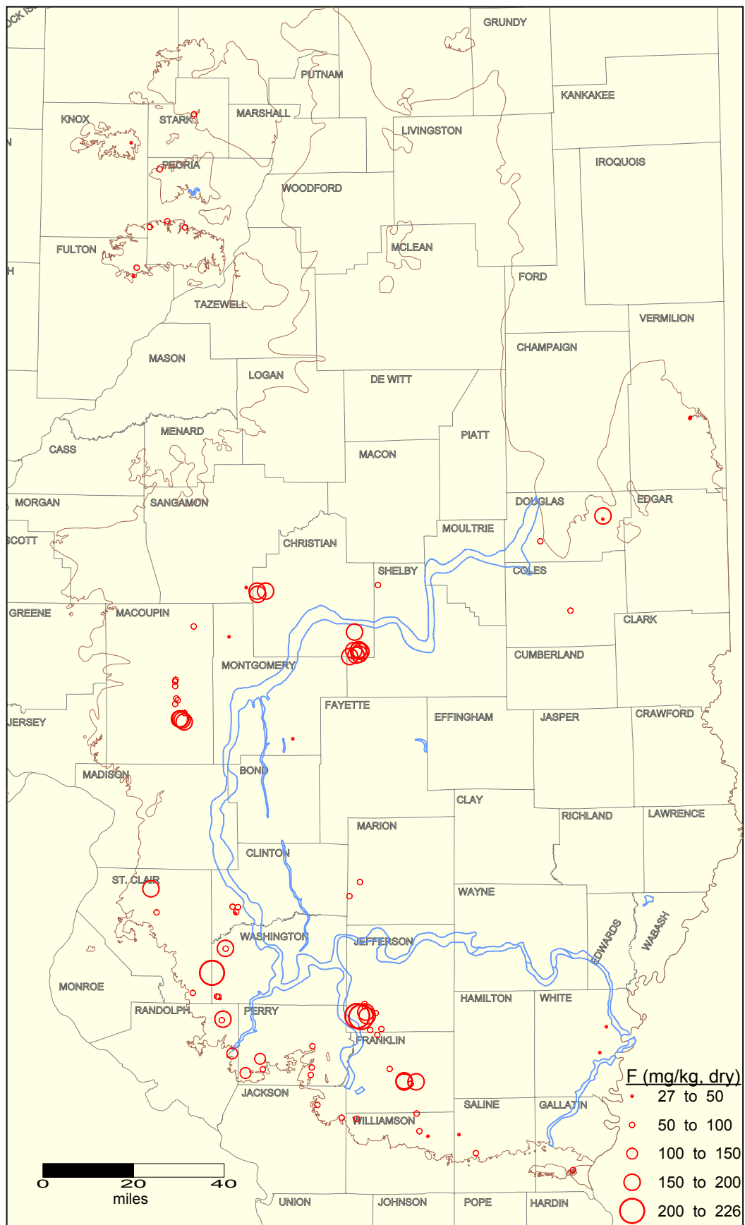
Fluorine concentration in Herrin Coal seam in Illinois. Brown and blue lines indicate the limit of the Herrin seam and Walshville channel, respectively.
