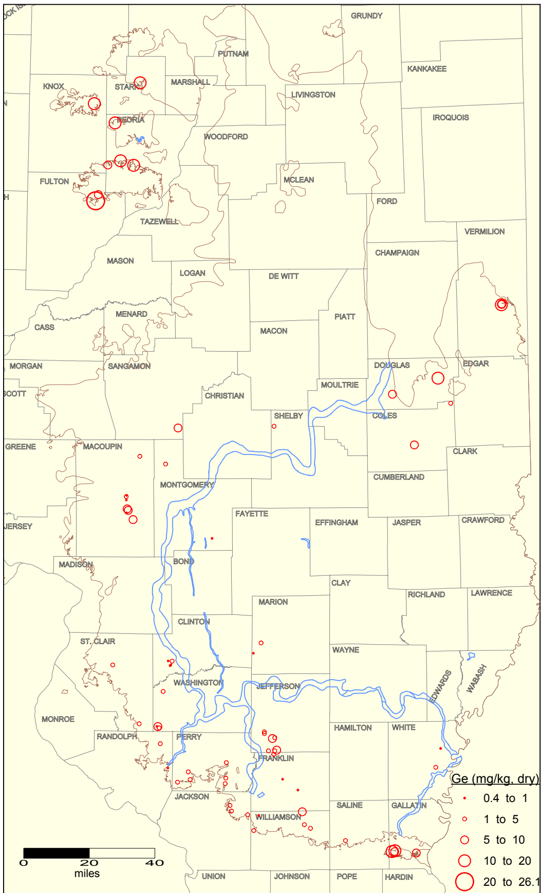
Germanium concentration in Herrin Coal seam in Illinois. Brown and blue lines indicate the limit of the Herrin seam and Walshville channel, respectively.
