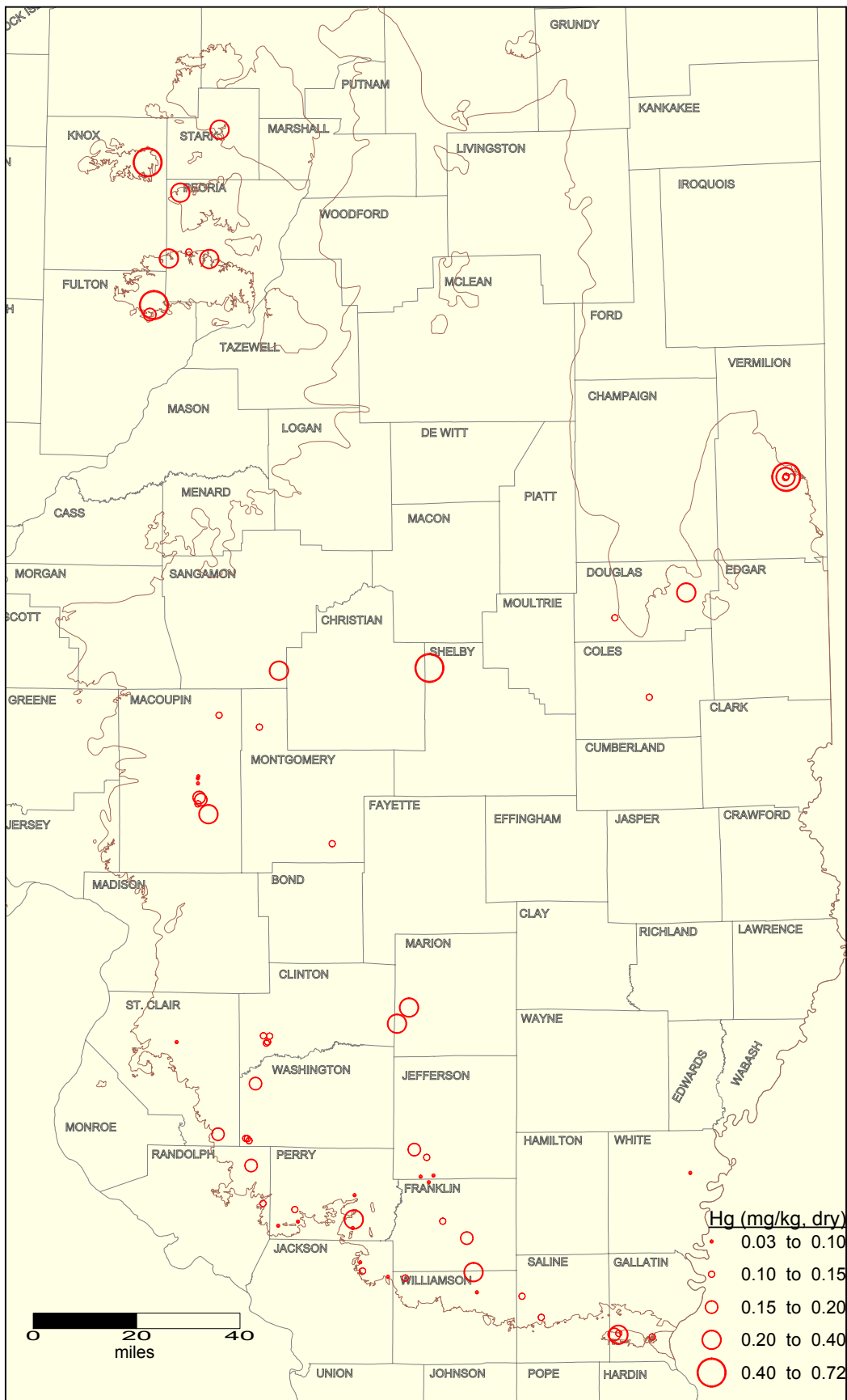
Mercury concentration in Herring Coal seam in Illinois. Brown and blue lines indicate the limit of the Herring seam and Walshville channel, respectively.
