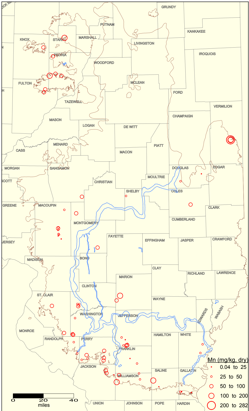
Manganese concentration in Herrin Coal seam in Illinois. Brown and blue lines indicate the limit of the Herrin seam and Walshville channel, respectively.
