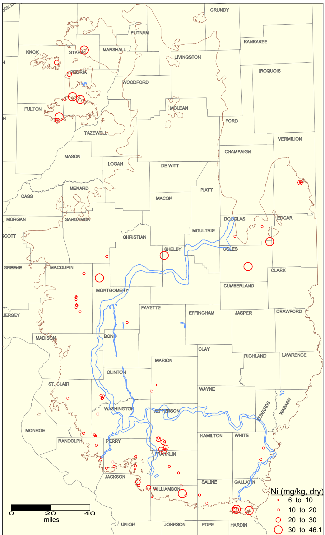
Nickel concentration in Herrin Coal seam in Illinois. Brown and blue lines indicate the limit of the Herrin seam and Walshville channel, respectively.
