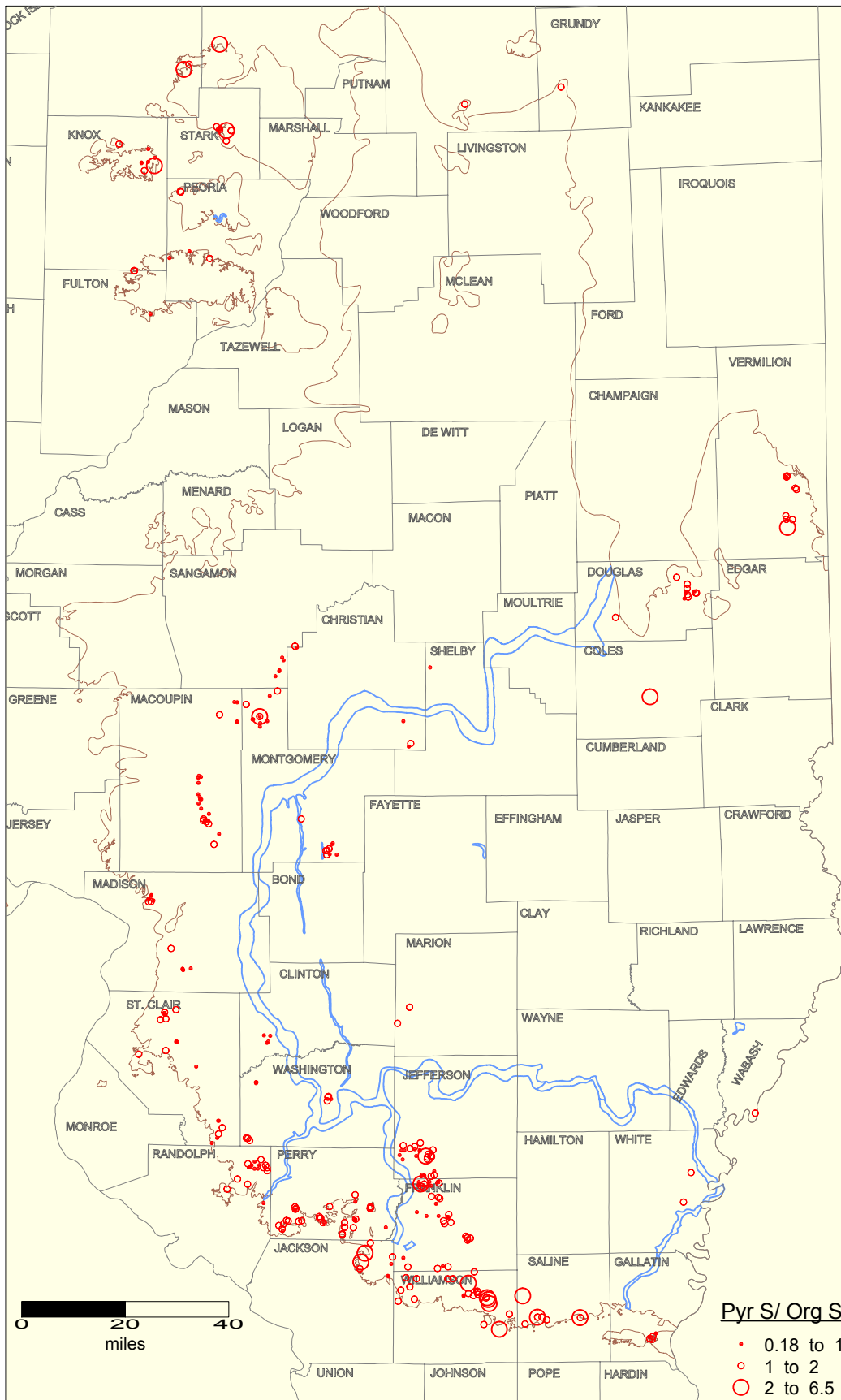
Pyritic sulfur content to organic sulfur content ratio in Herrin Coal seam in Illinois. Brown and blue lines indicate the limit of the Herrin seam and Walshville channel, respectively.
