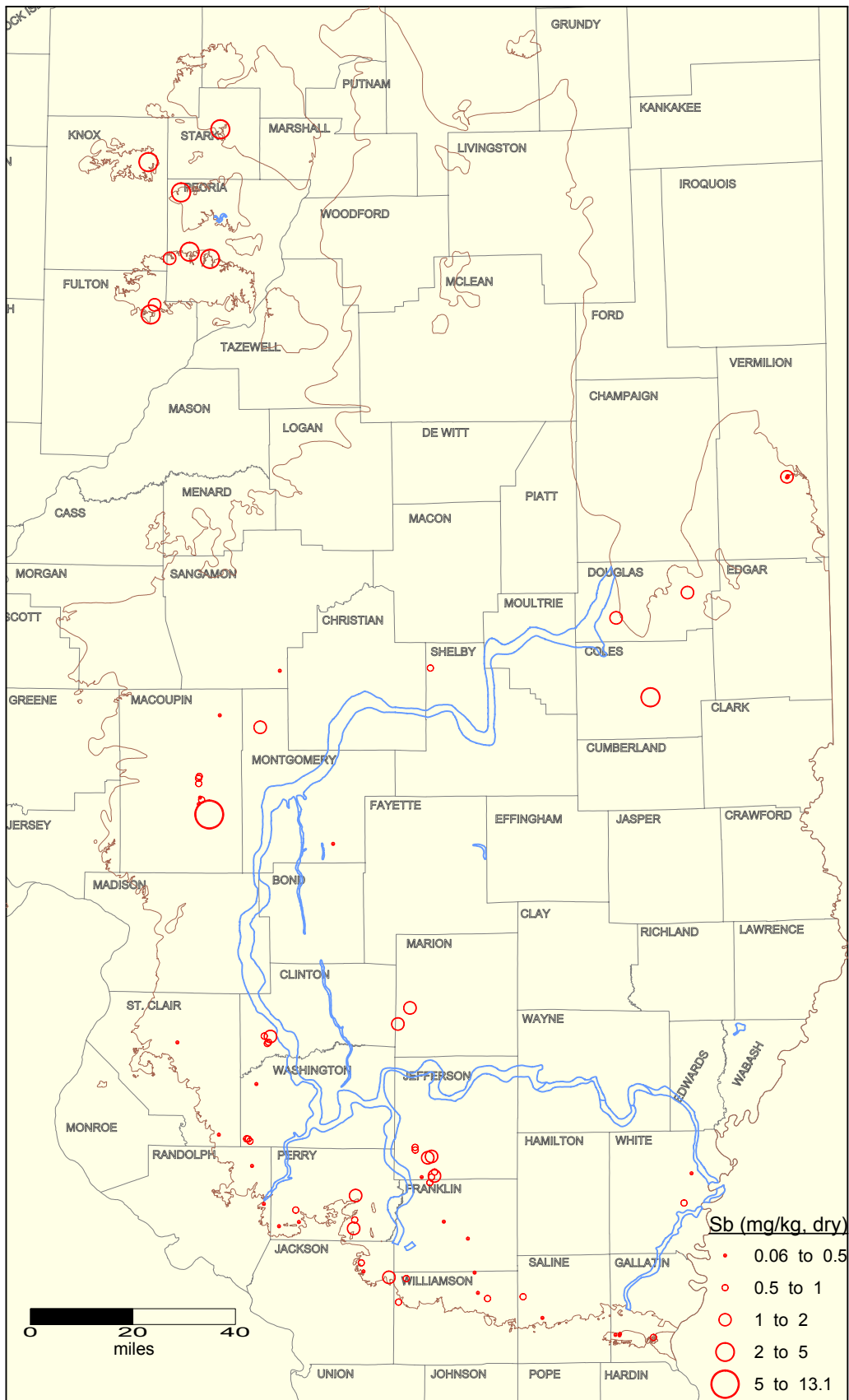
Antimony concentration in Herrin Coal seam in Illinois. Brown and blue lines indicate the limit of the Herrin seam and Walshville channel, respectively.
