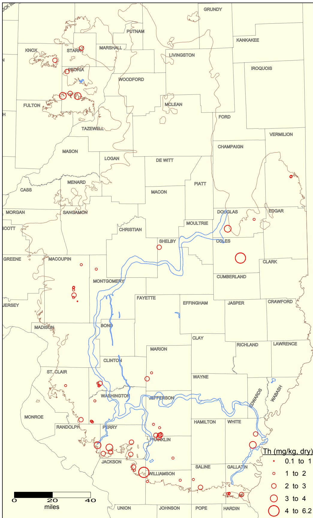
Thorium concentration in Herrin Coal seam in Illinois. Brown and blue lines indicate the limit of the Herrin seam and Walshville channel, respectively.
