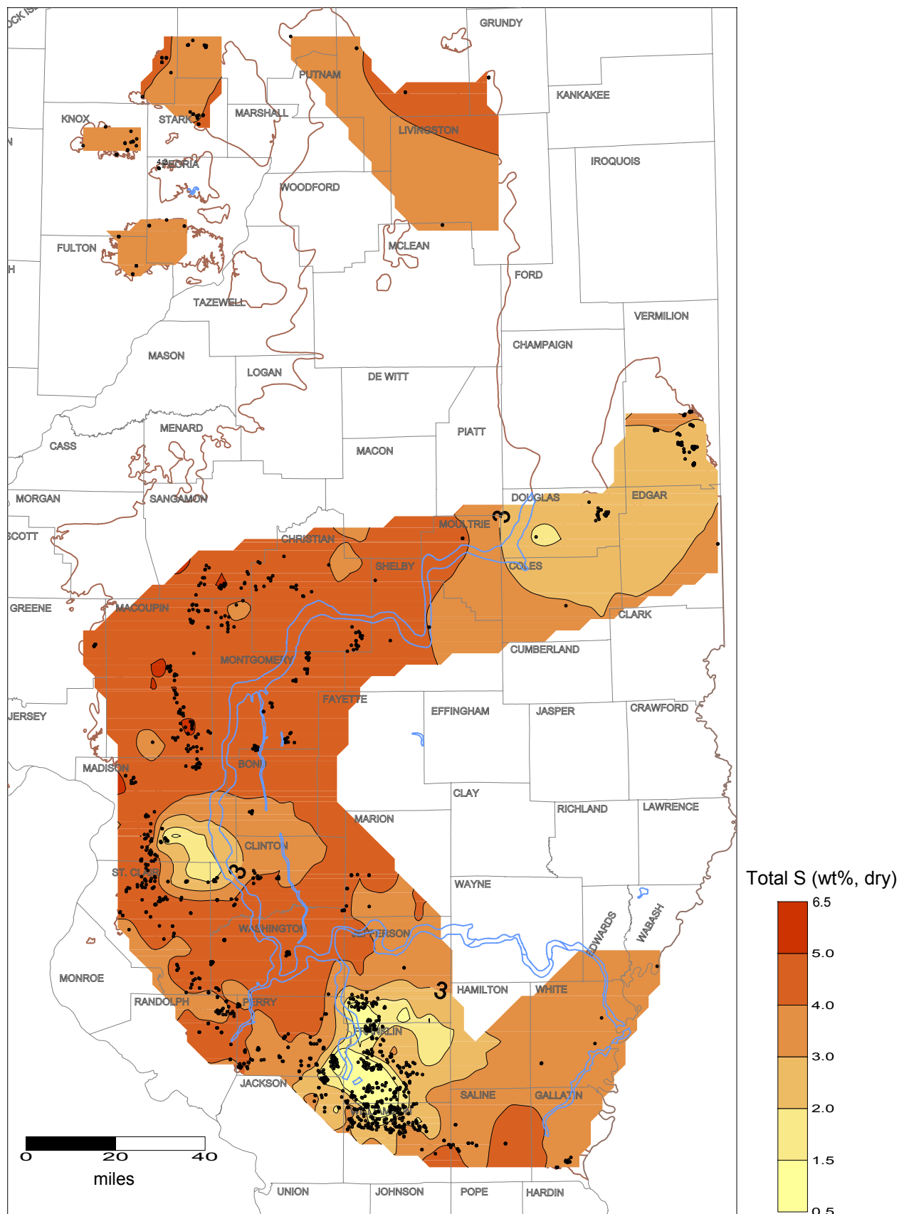
Total sulfur content of Herrin Coal seam in Illinois. Black solid circles indicate sample locations. Brown and blue lines indicate the limit of the Herrin seam and Walshville channel, respectively.
