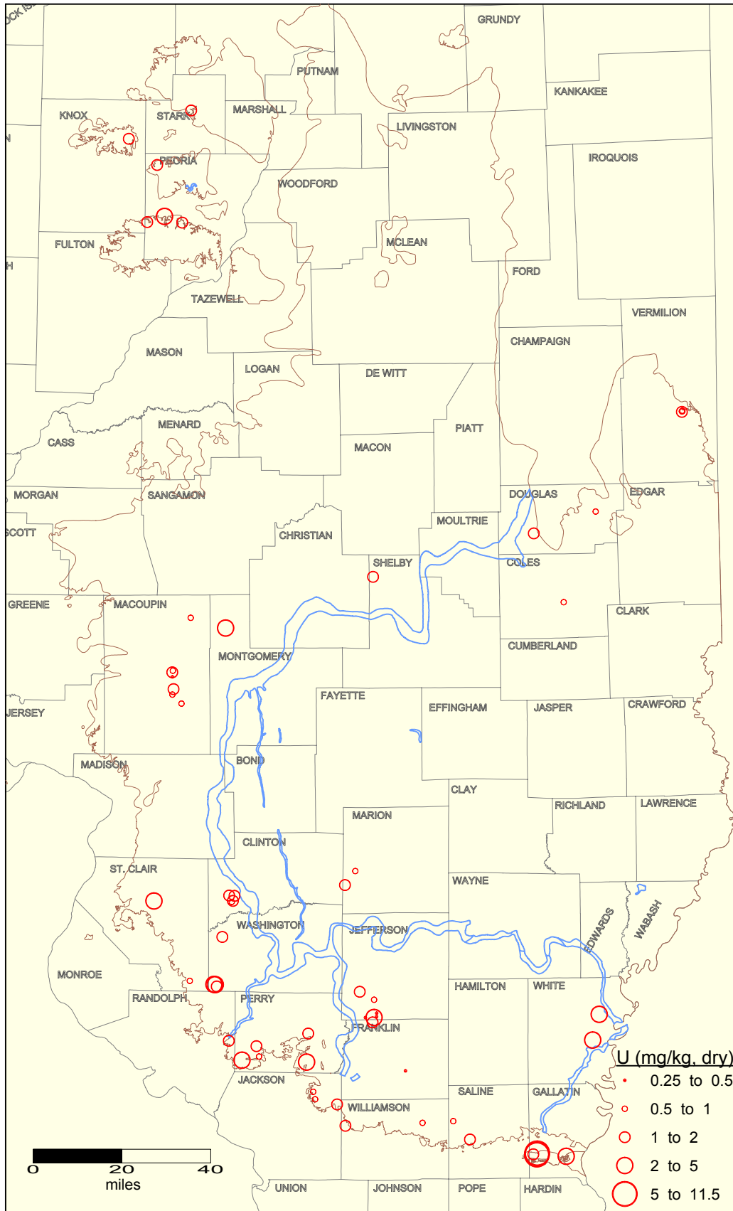
Uranium concentration in Herrin Coal seam in Illinois. Brown and blue lines indicate the limit of the Herrin seam and Walshville channel, respectively.
