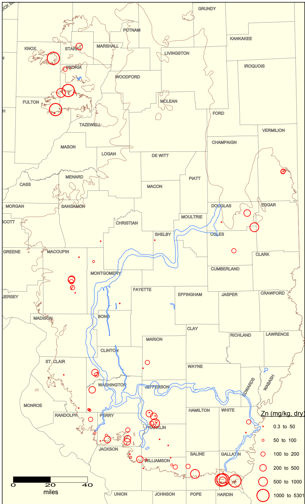
Zinc concentration in Herrin Coal seam in Illinois. Brown and blue lines indicate the limit of Herrin seam and Walshville channel, respectively.
