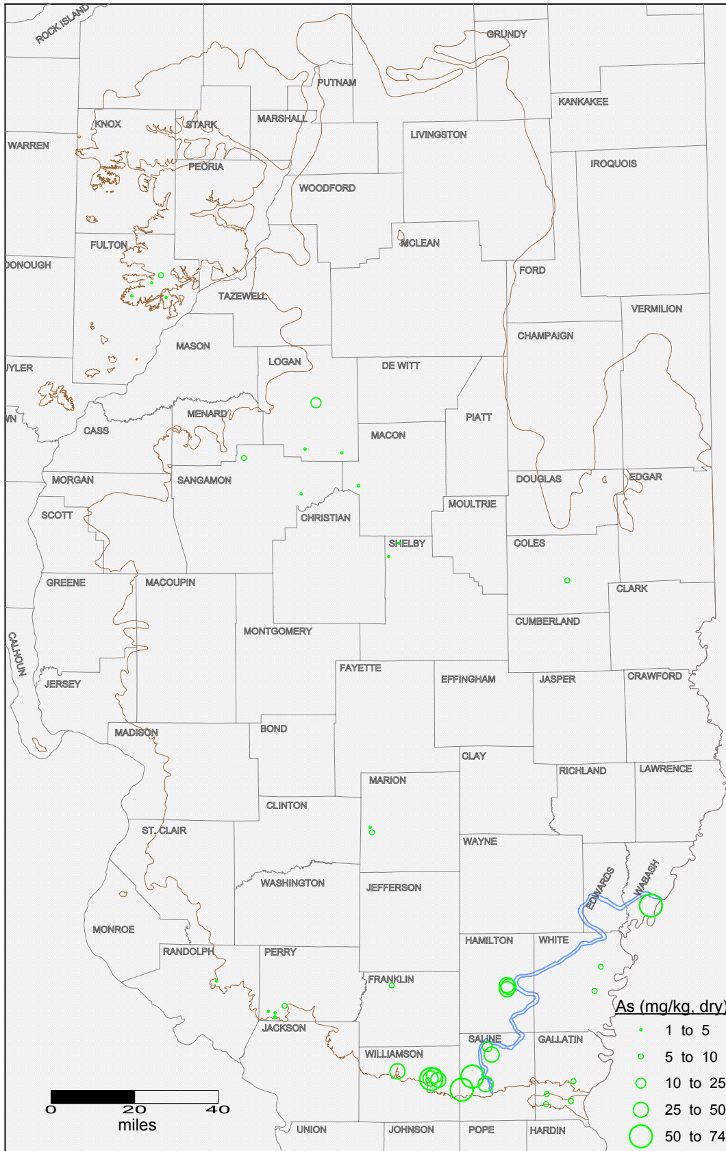
Arsenic concentration in Springfield Coal seam in Illinois. Brown and blue lines indicate the limit of the Springfield seam and Galatia channel, respectively.
