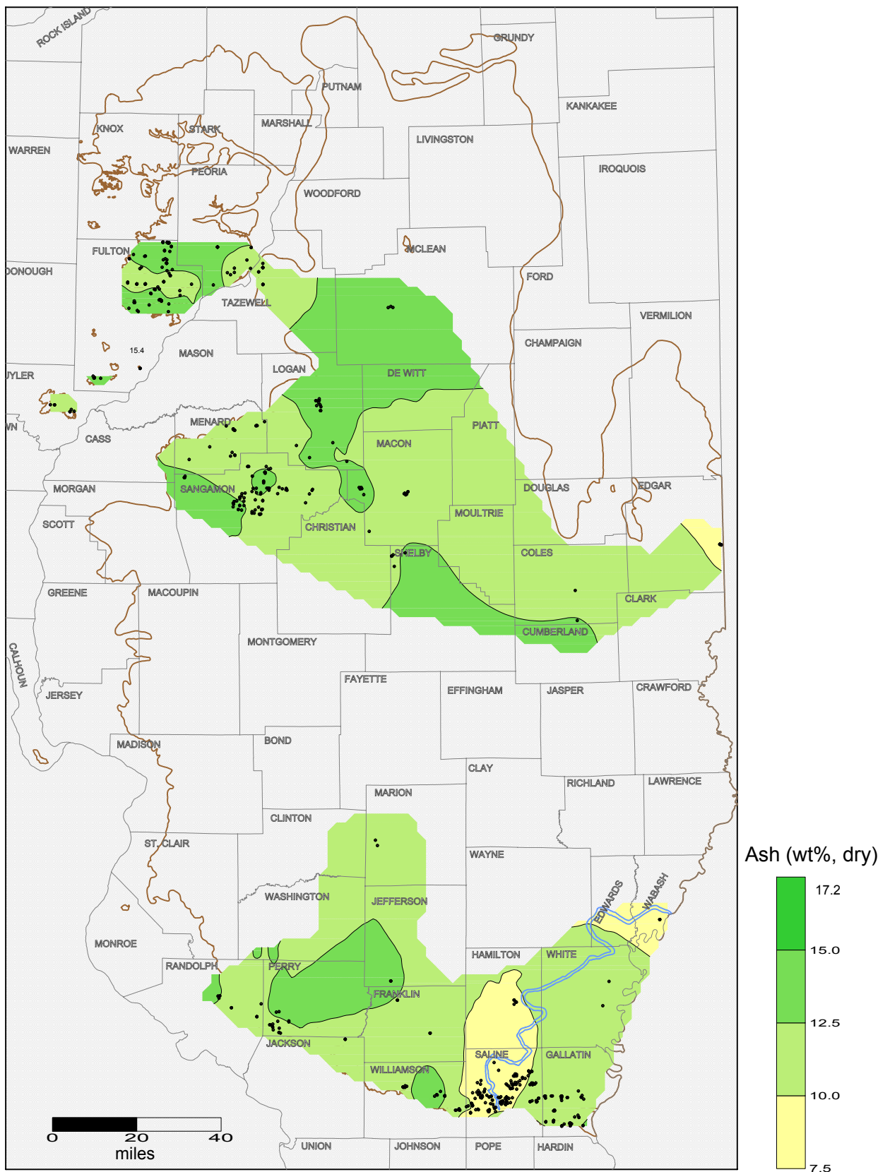
Ash yield of Springfield Coal seam in Illinois. Black solid circles indicate sample locations. Brown and blue lines indicate the limit of the Springfield seam and Galatia channel, respectively.
