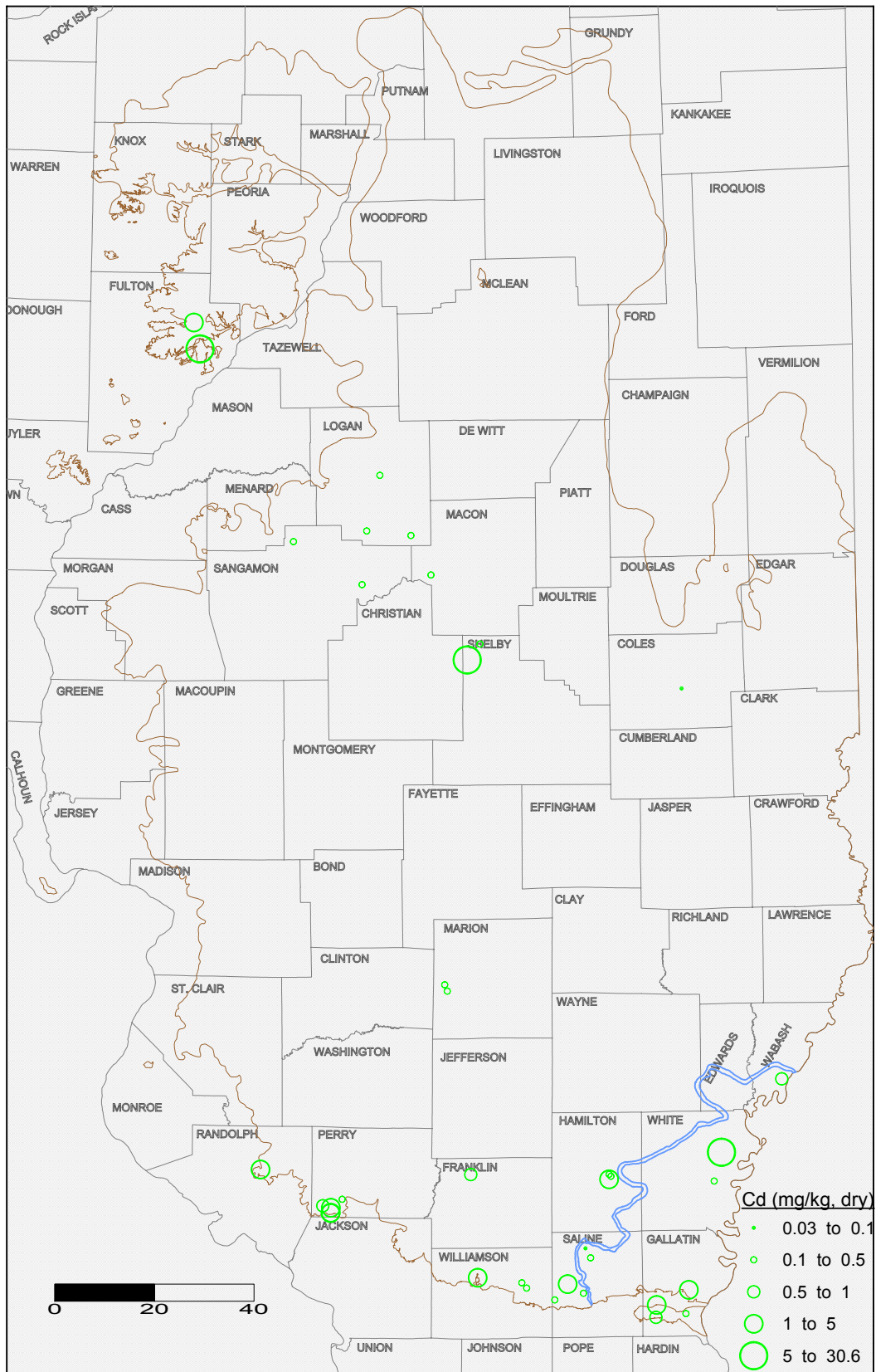
Cadmium concentration in Springfield Coal seam in Illinois. Brown and blue lines indicate the limit of the Springfield seam and Galatia channel, respectively.
