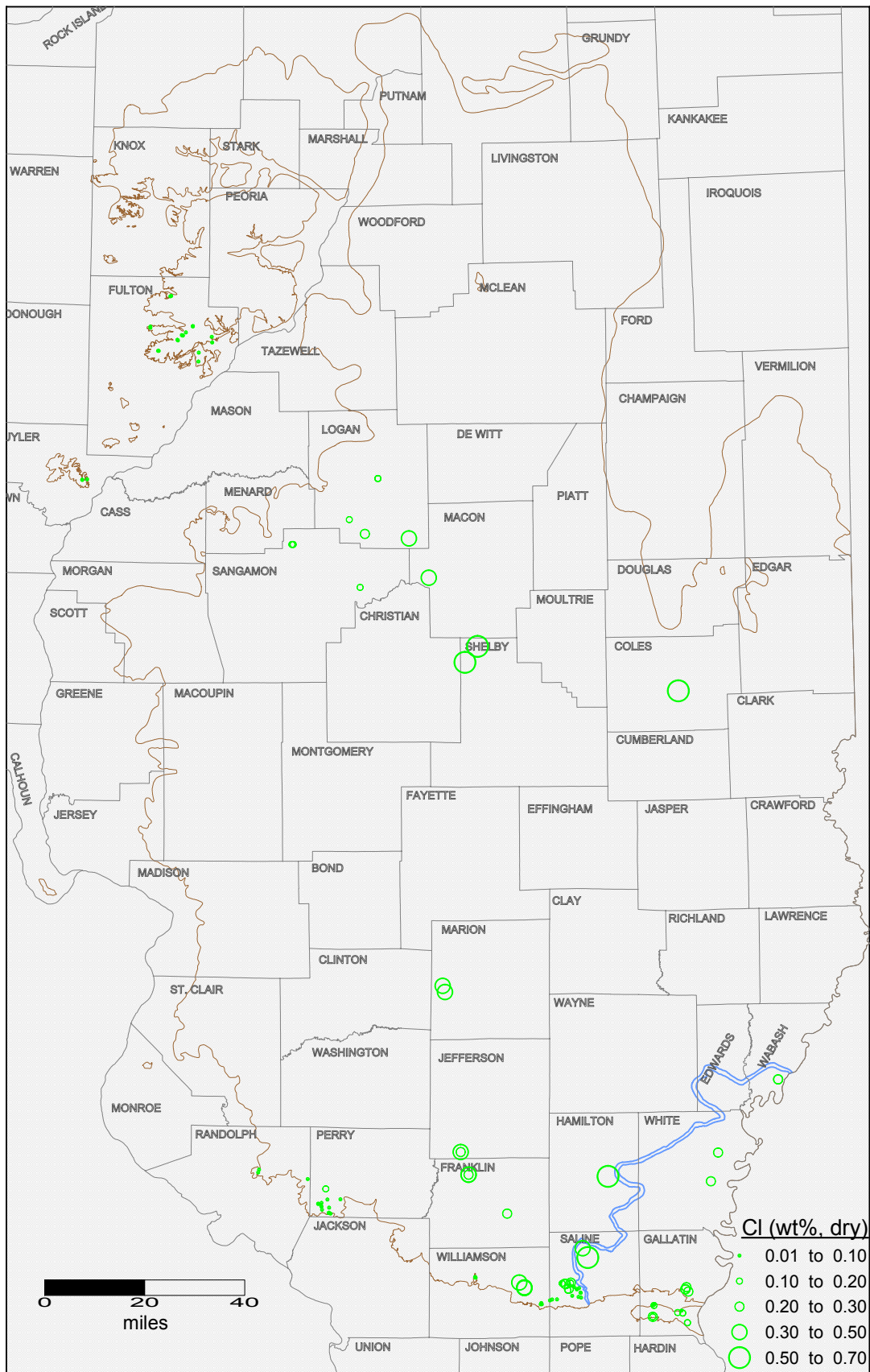
Chlorine content of Springfield Coal seam in Illinois. Brown and blue lines indicate the limit of the Springfield seam and Galatia channel, respectively.
