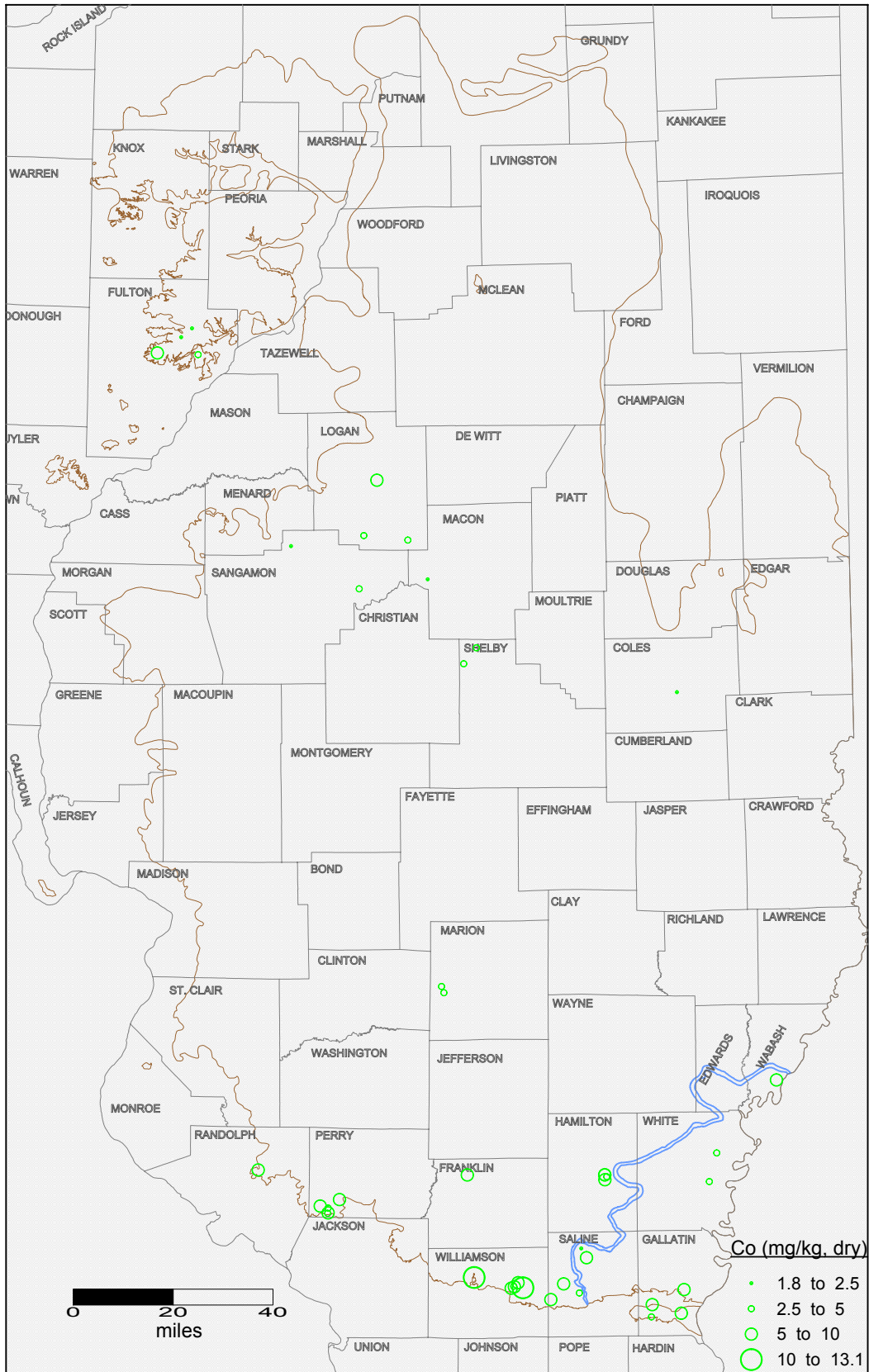
Cobalt concentration in Springfield Coal seam in Illinois. Brown and blue lines indicate the limit of the Springfield seam and Galatia channel, respectively.
