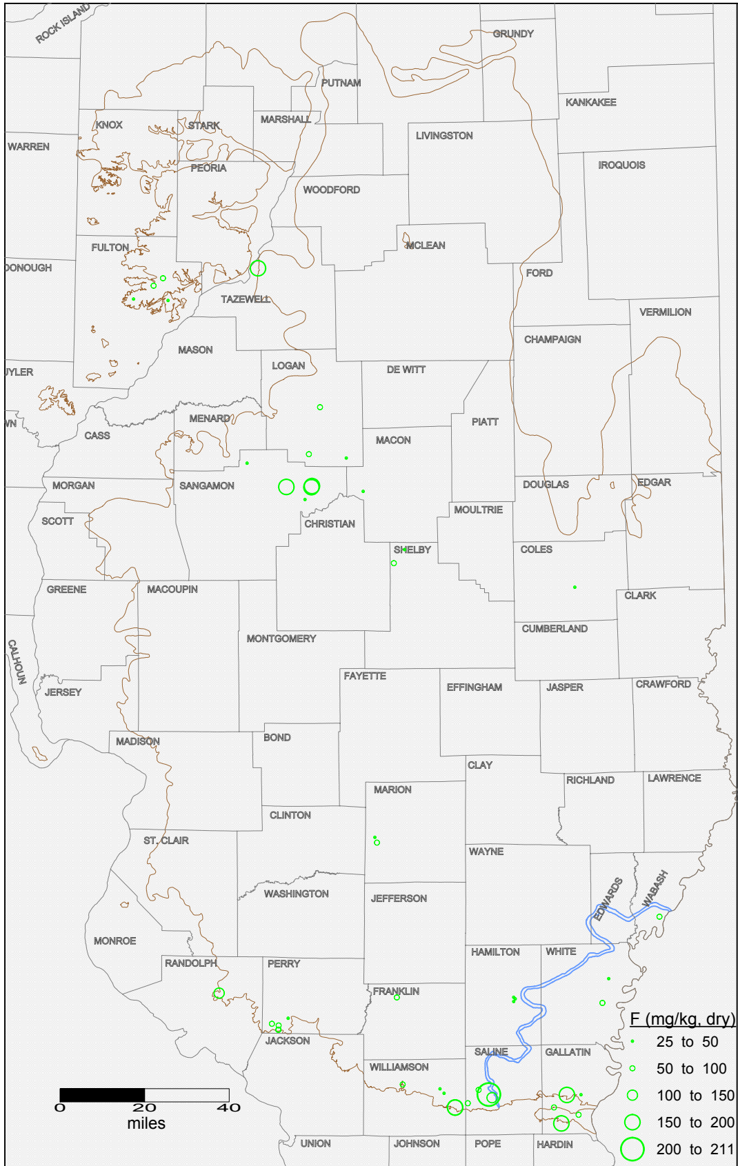
Fluorine concentration in Springfield Coal seam in Illinois. Brown and blue lines indicate the limit of the Springfield seam and Galatia channel, respectively.
