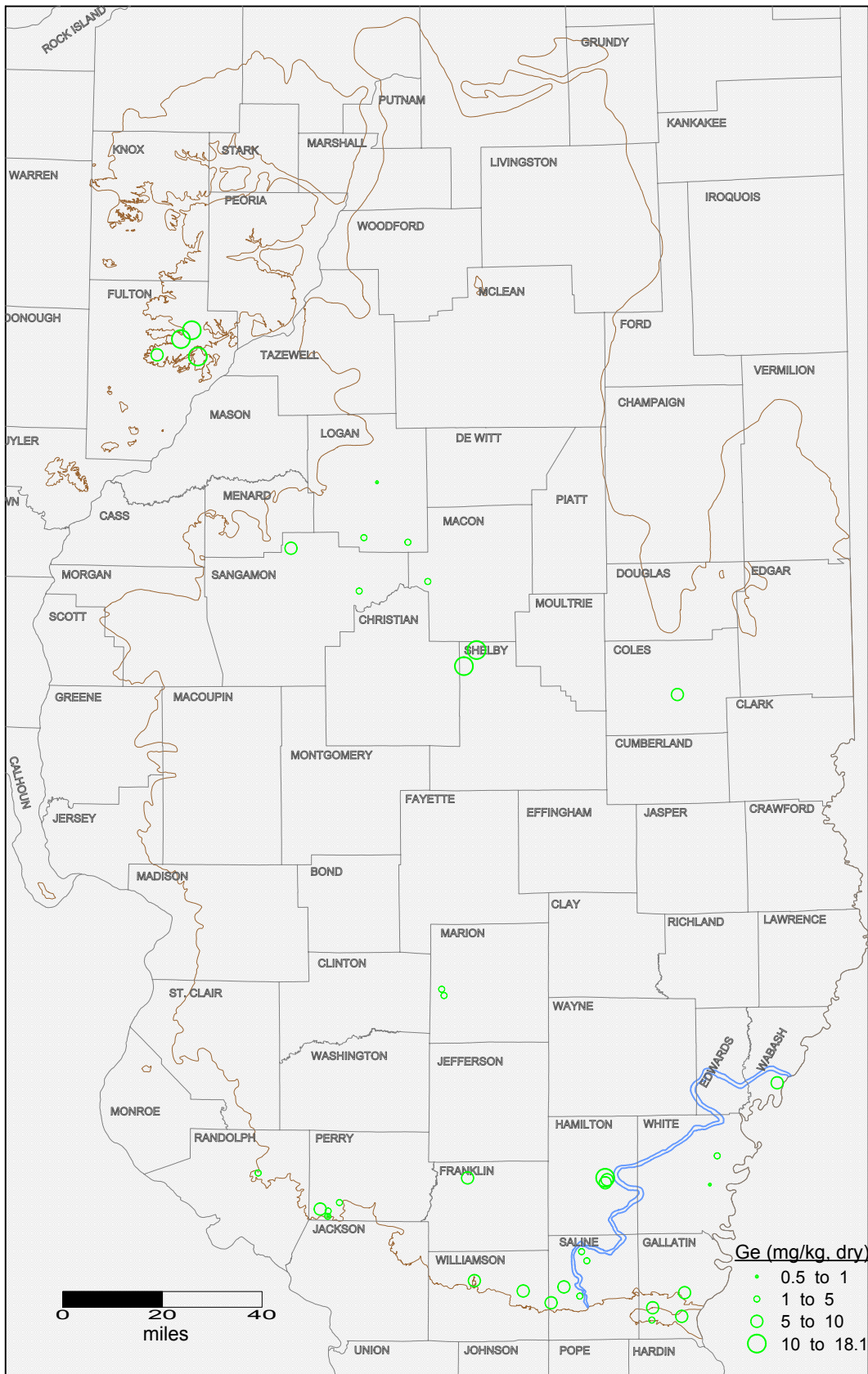
Germanium concentration in Springfield Coal seam in Illinois. Brown and blue lines indicate the limit of the Springfield seam and Galatia channel, respectively.
