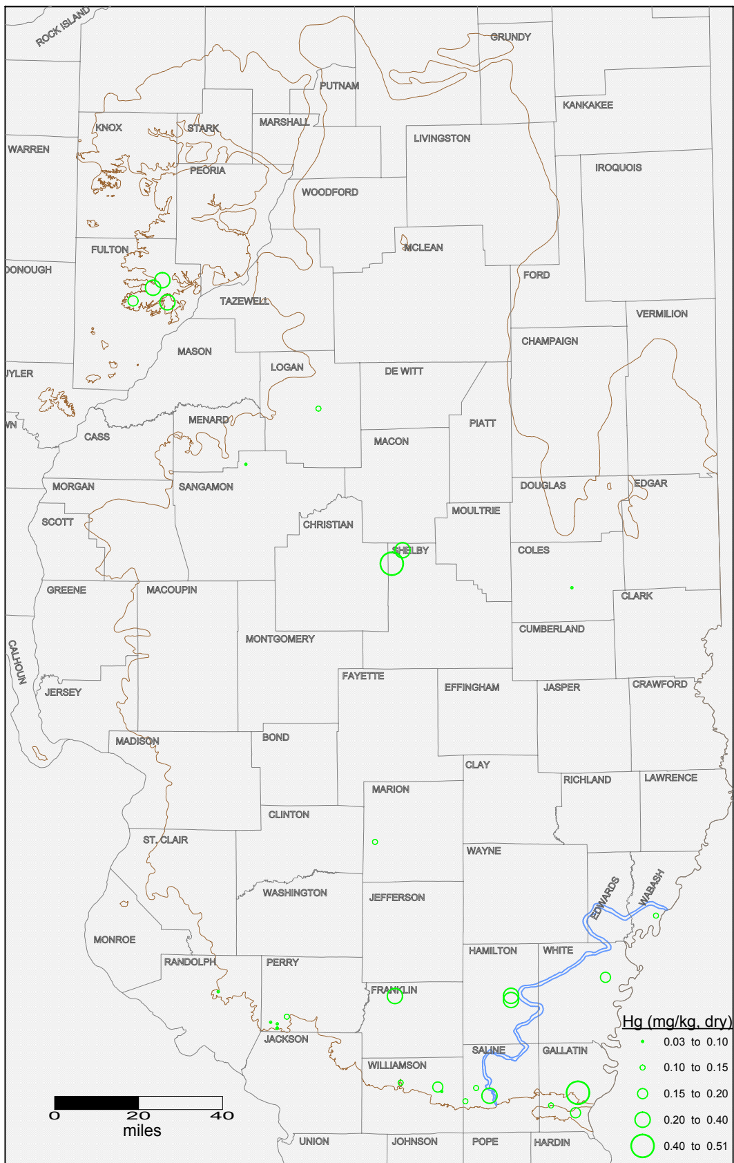
Mercury concentration in Springfield Coal seam in Illinois. Brown and blue lines indicate the limit of the Springfield seam and Galatia channel, respectively.
