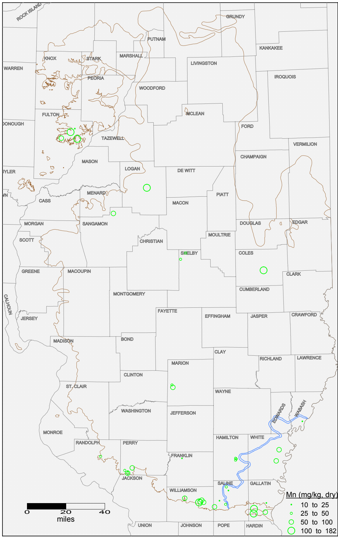
Manganese concentration in Springfield Coal seam in Illinois. Brown and blue lines indicate the limit of the Springfield seam and Galatia channel, respectively.
