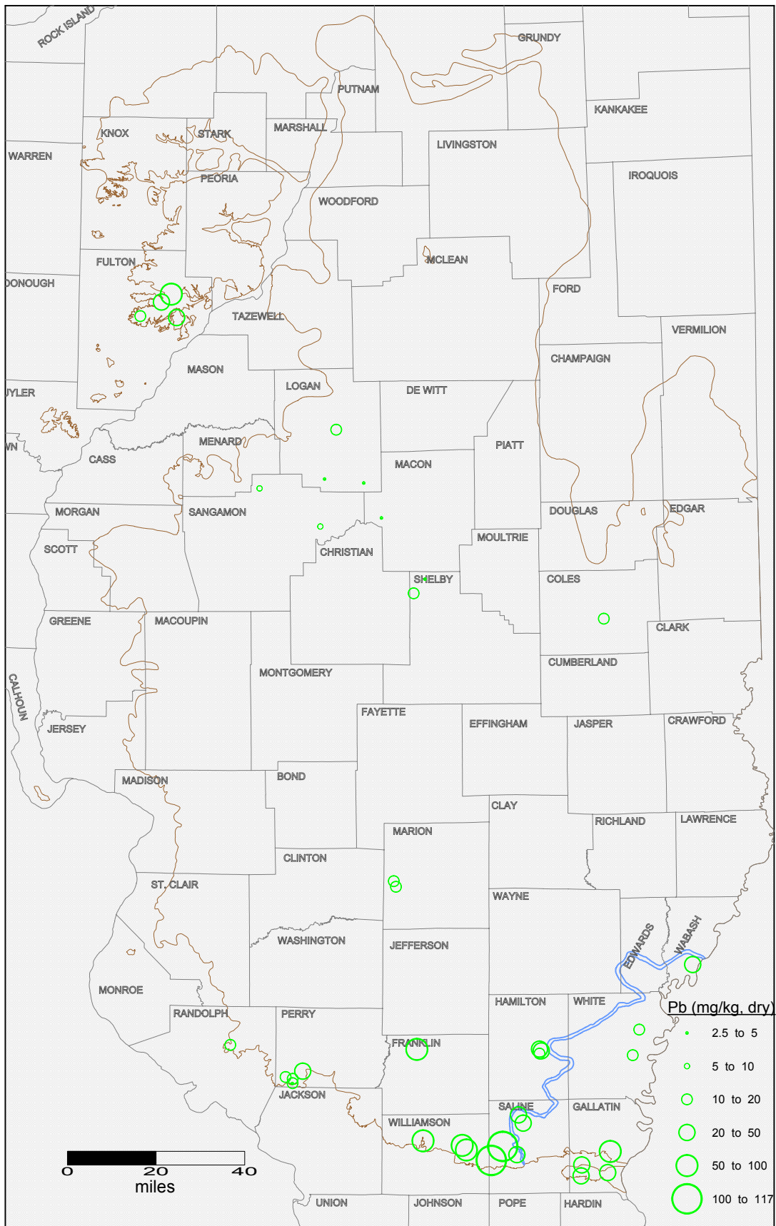
Lead concentration in Springfield Coal seam in Illinois. Brown and blue lines indicate the limit of the Springfield seam and Galatia channel, respectively.
