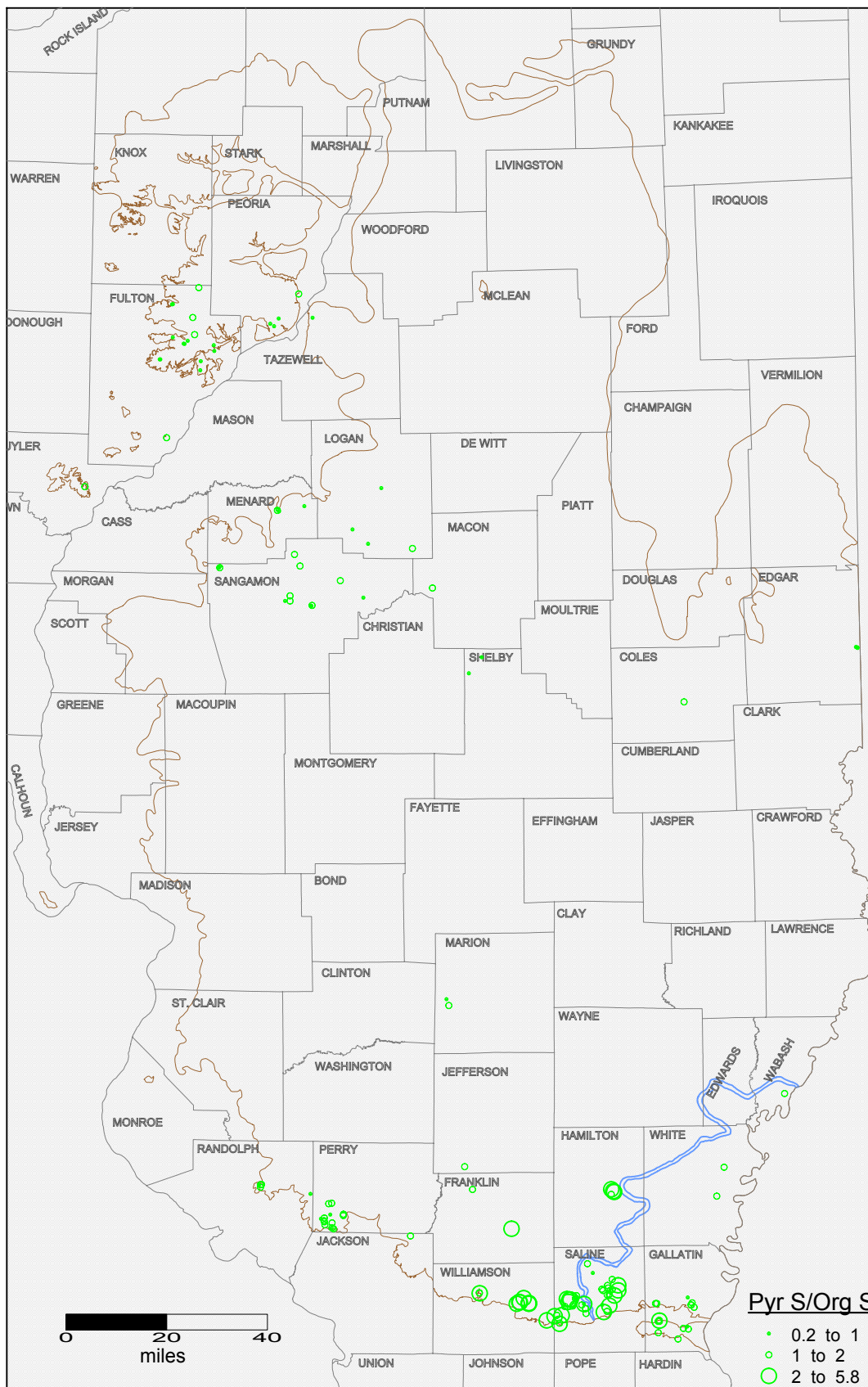
Pyritic sulfur content to organic sulfur content ratio in Springfield Coal seam in Illinois. Brown and blue lines indicate the limit of the Springfield seam and Galatia channel, respectively.
