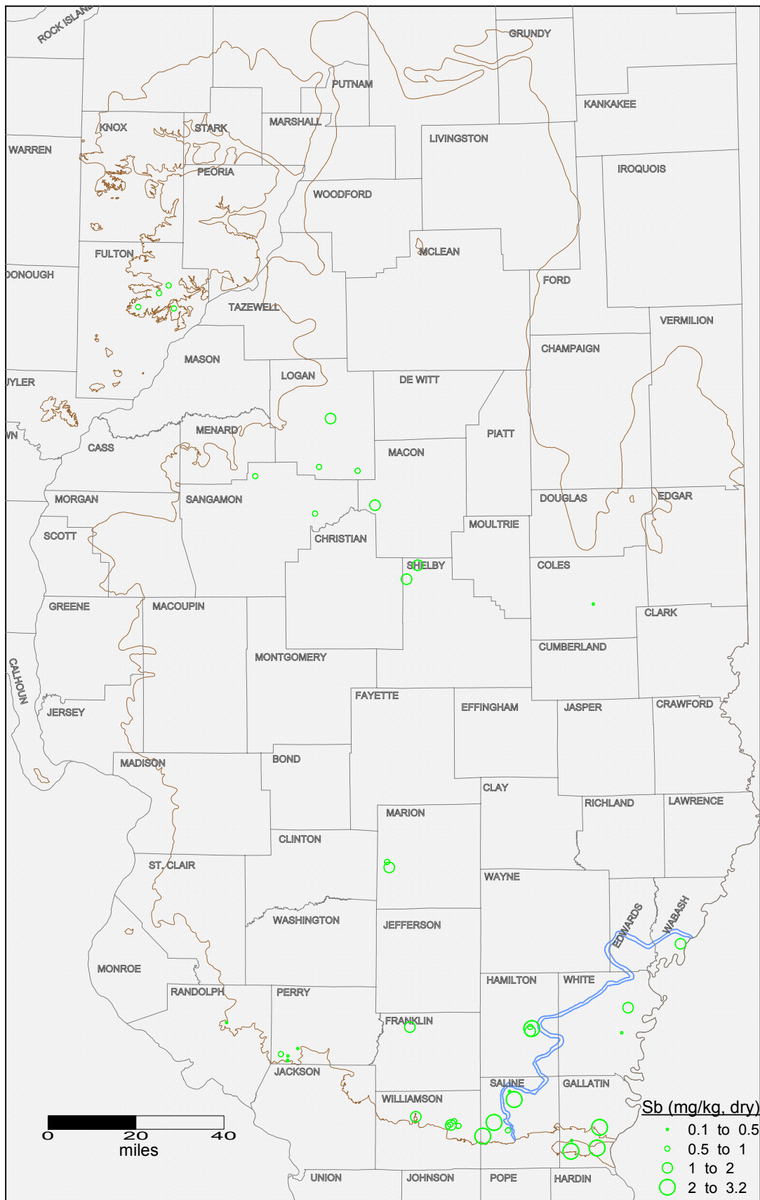
Antimony concentration in Springfield Coal seam in Illinois. Brown and blue lines indicate the limit of the Springfield seam and Galatia channel, respectively.
