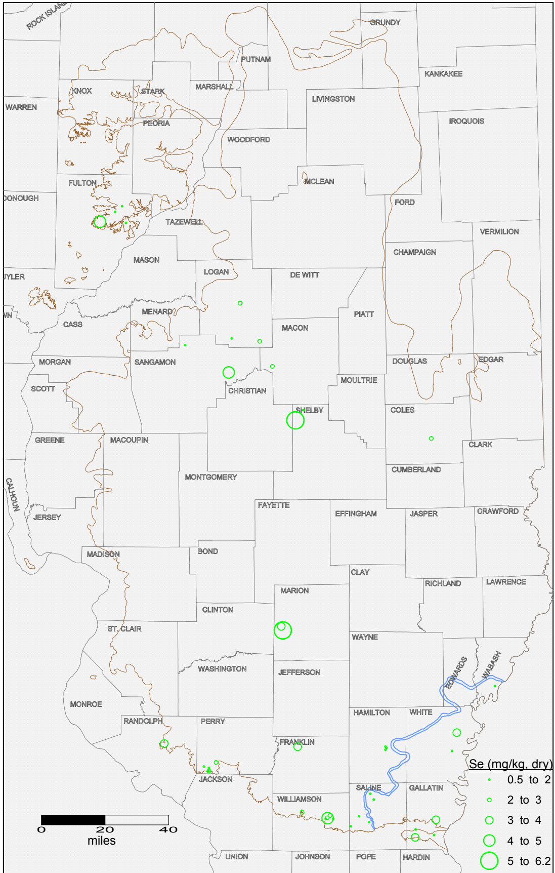
Selenium concentration in Springfield Coal seam in Illinois. Brown and blue lines indicate the limit of the Springfield seam and Galatia channel, respectively.
