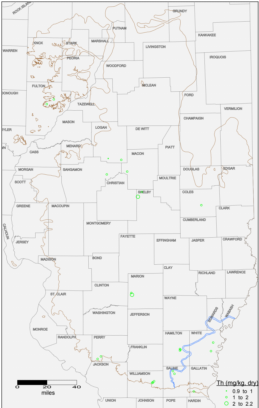
Thorium concentration in Springfield Coal seam in Illinois. Brown and blue lines indicate the limit of the Springfield seam and Galatia channel, respectively.
