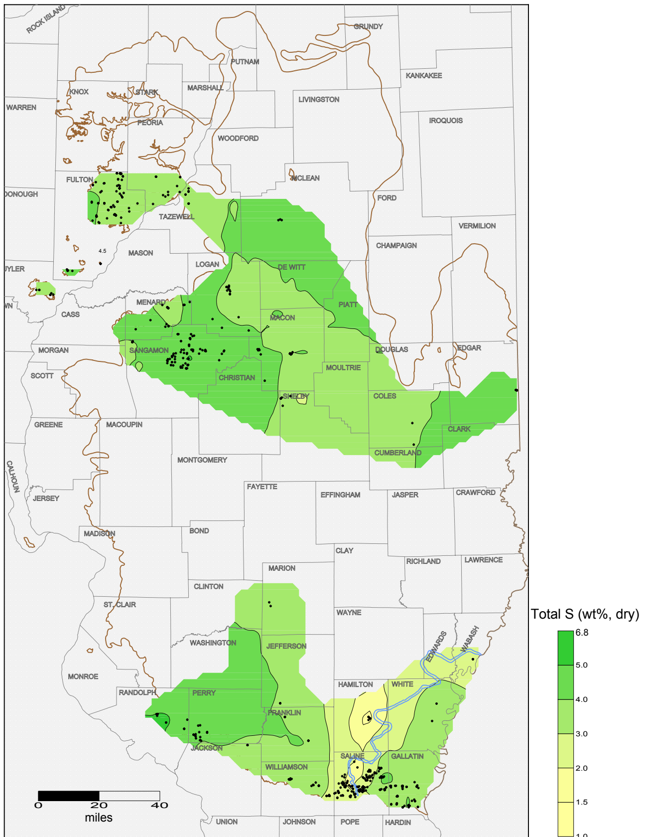
Total sulfur content of Springfield Coal seam in Illinois. Black solid circles indicate sample locations. Brown and blue lines indicate the limit of the Springfield seam and Galatia channel, respectively.
