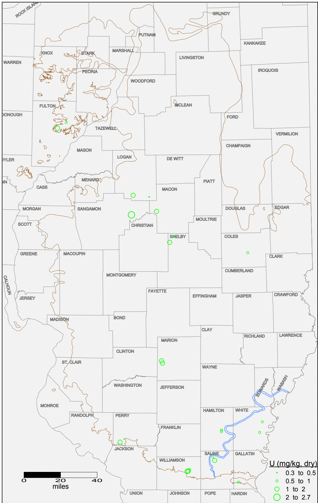
Uranium concentration in Springfield Coal seam in Illinois. Brown and blue lines indicate the limit of the Springfield seam and Galatia channel, respectively.
