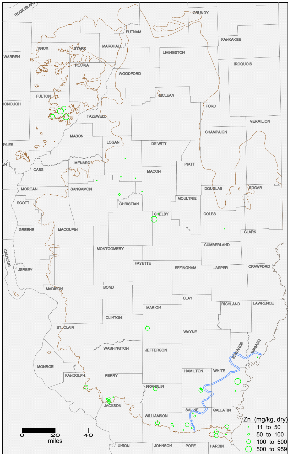
Zinc concentration in Springfield Coal seam in Illinois. Brown and blue lines indicate the limit of the Springfield seam and Galatia channel, respectively.
